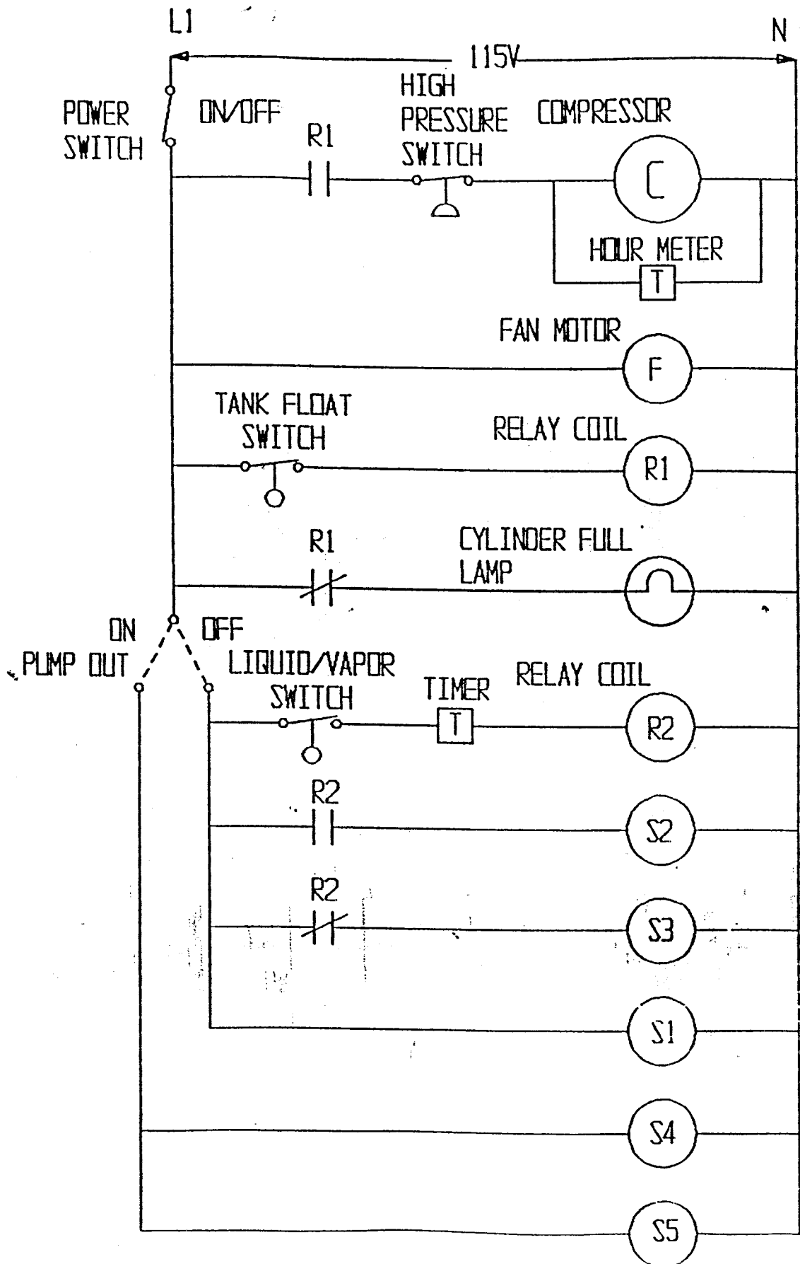
RECOVER/RECYCLING UNIT WIRING DIAGRAM
